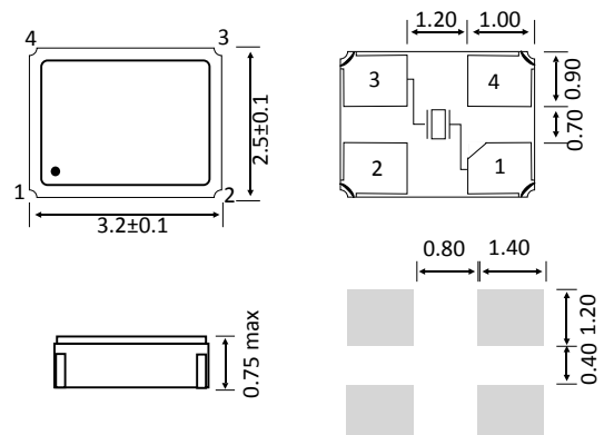
Dimensions (mm)
